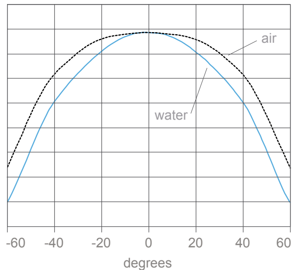
Beam Angle
